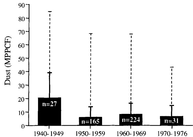
FIGURE 1. Mean midget impinger dust measurements by decade for the Leadville molybdenum mine, with standard deviation (unbroken line) and highest recorded value (dashed line) expressed in million particles per cubic foot (MPPCF).
